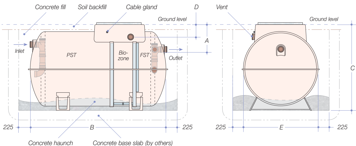
All dimensions in millimetres. PST = Primary Settlement Tank; Biozone = Biological Treatment Zone; FST = Final Settlement Tank.
